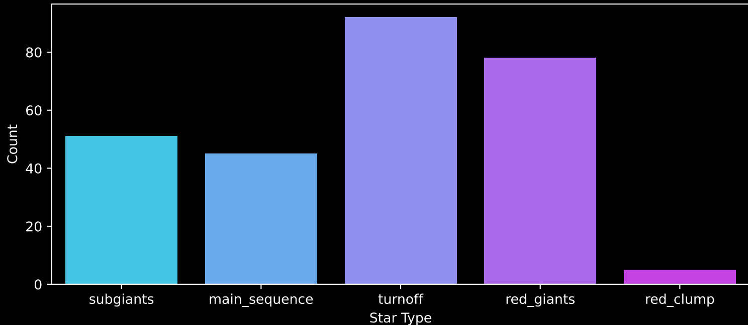
GALAH DR4 Field: [9395] Count plot of Star Type
