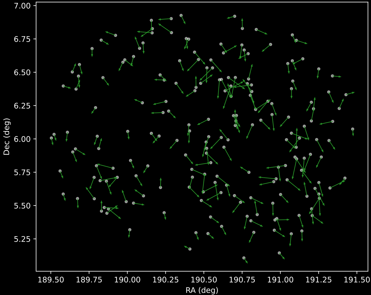
GALAH DR4 Cluster 4 Proper Motion Vectors (n=194)
