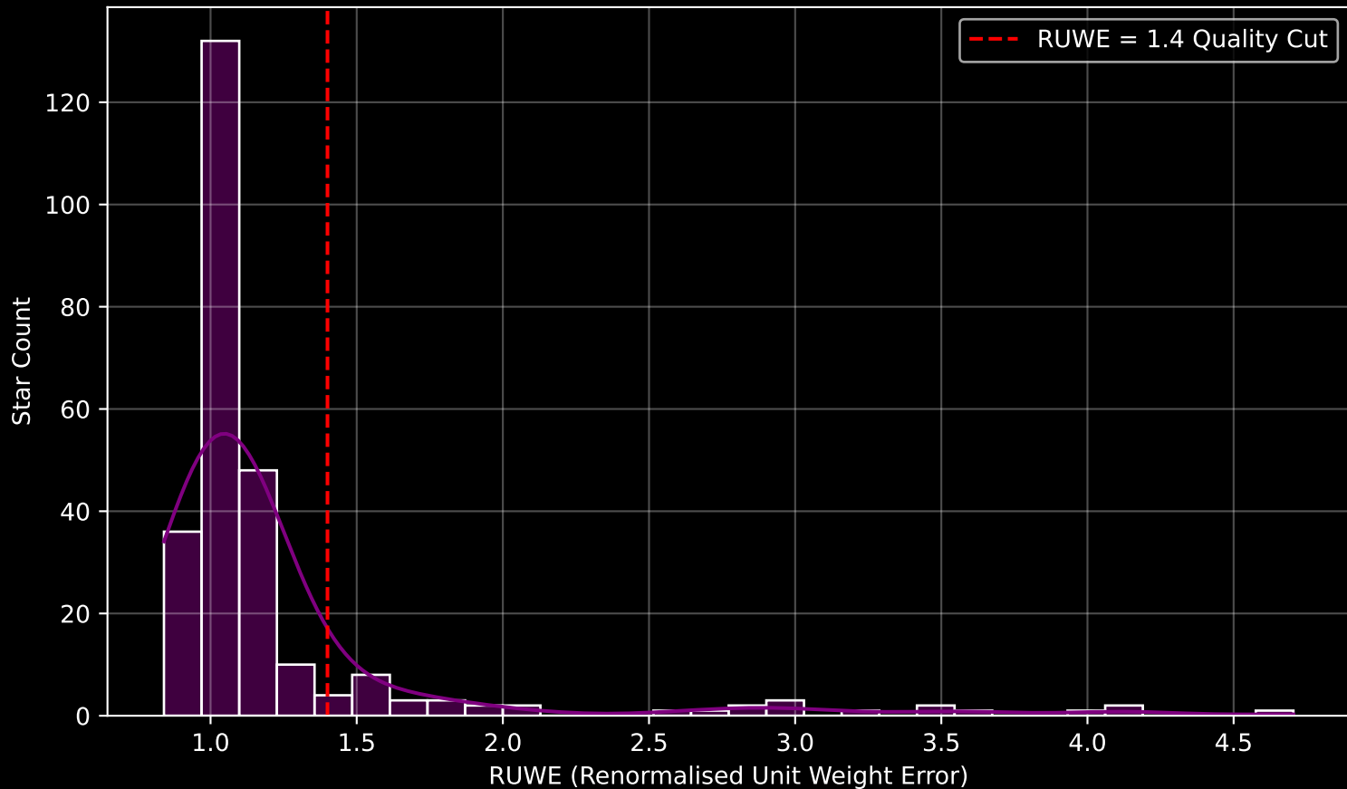
GALAH DR4 Field [9395] RUWE Distribution (n= 263)
