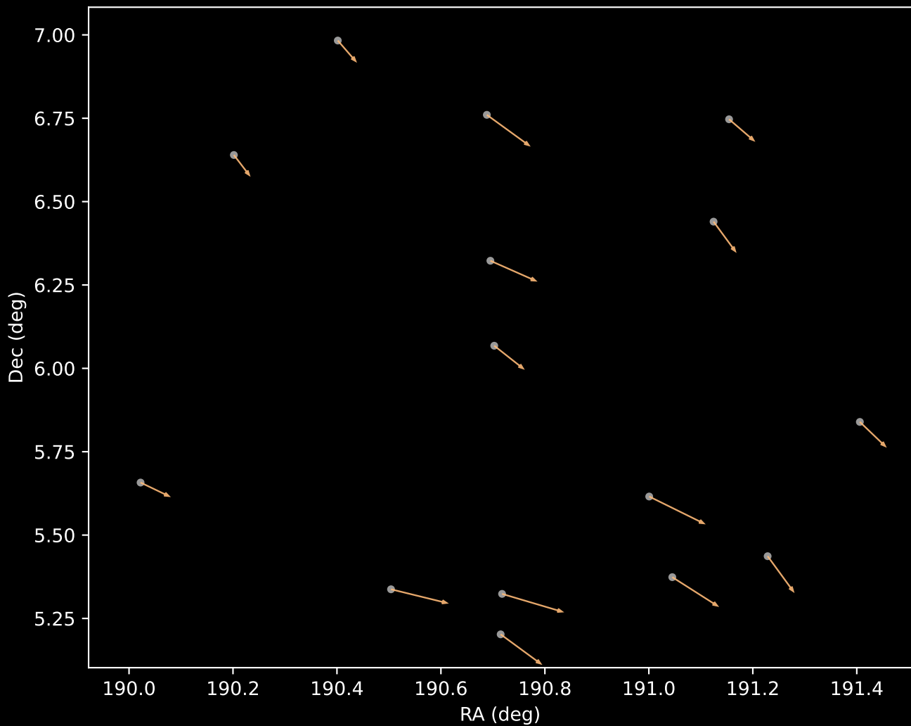
GALAH DR4 Cluster 3 Proper Motion Vectors (n=15)
